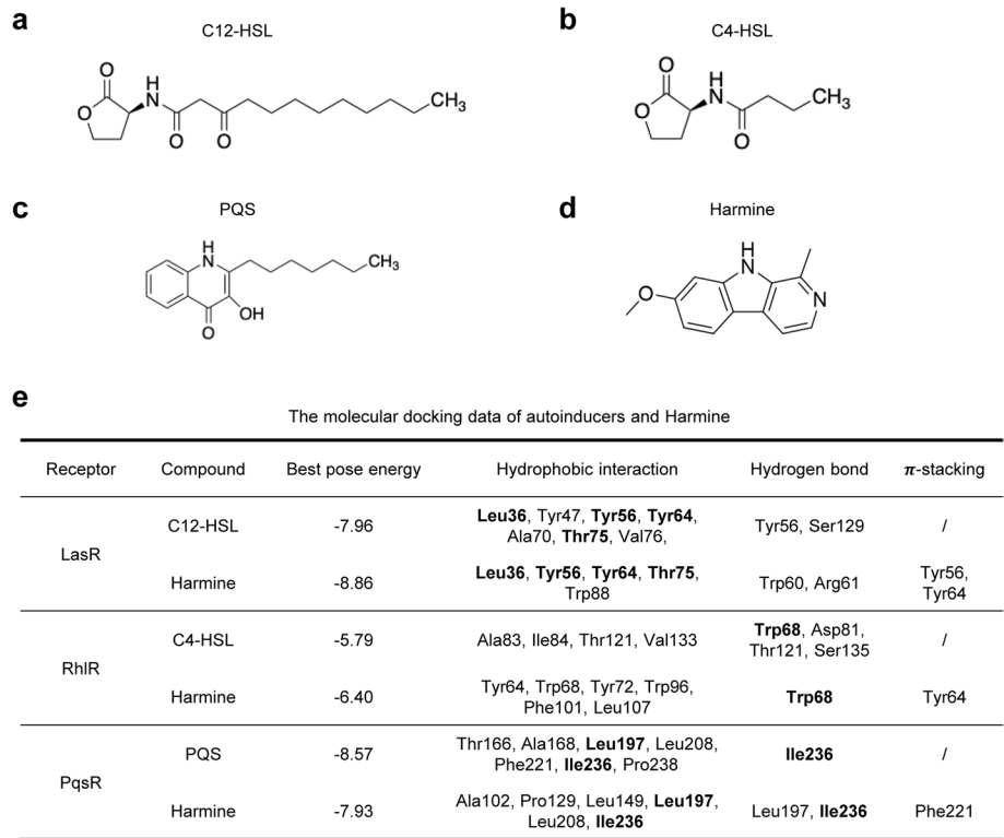
Fig. 1 Structures of molecules and data of molecular docking. The structures of autoinducers C12-HSL (a), C4-HSL (b), and PQS (c); and the structure of Harmine (d). The molecular docking data (e) of autoinducers and Harmine with LasR , RhlR , and PqsR , respectively
