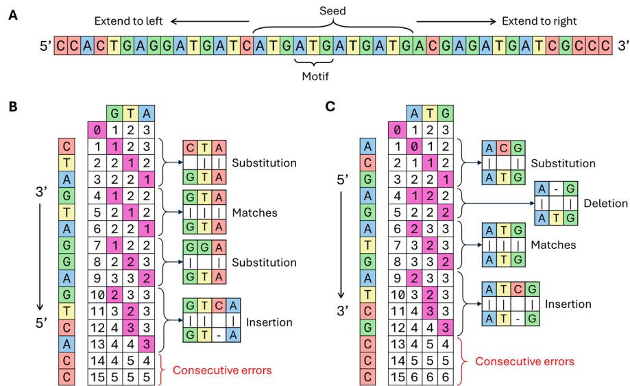
Fig. 1 The overview of pytrf algorithm. A the found seed repeat sequence and motif sequence before extending to both left and right. B extending repeat sequence to left by aligning sequence to the reversed motif sequence using wraparound dynamic programming to calculate edit distance. C extending repeat sequence to right
