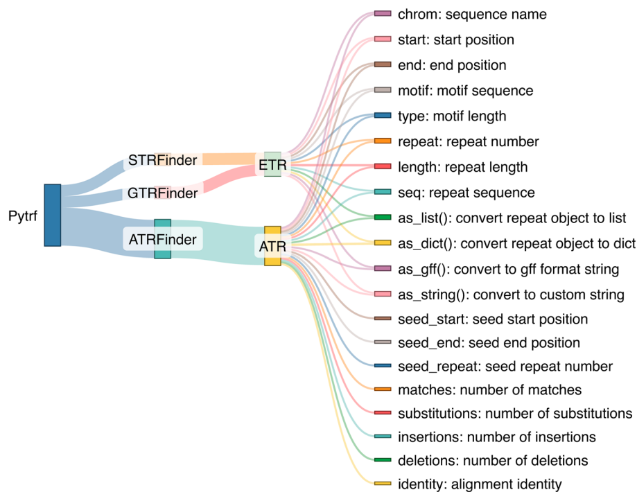
Fig. 2 The class structures of pytrf and their properties and methods
