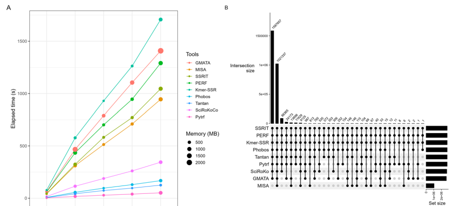
Fig. 3 The performance comparison for finding perfect microsatellites. A comparison of elapsed time and peak memory usage. B upset plot for intersections of search results
