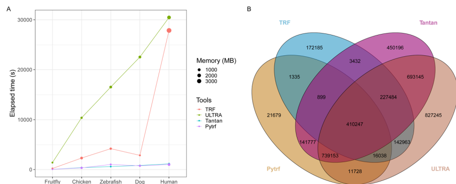
Fig. 5 The performance comparison for finding approximate tandem repeats with motif size of 1–100 bp. A comparison of elapsed time and peak memory usage. B venn plot for showing number of intersections between different tools
