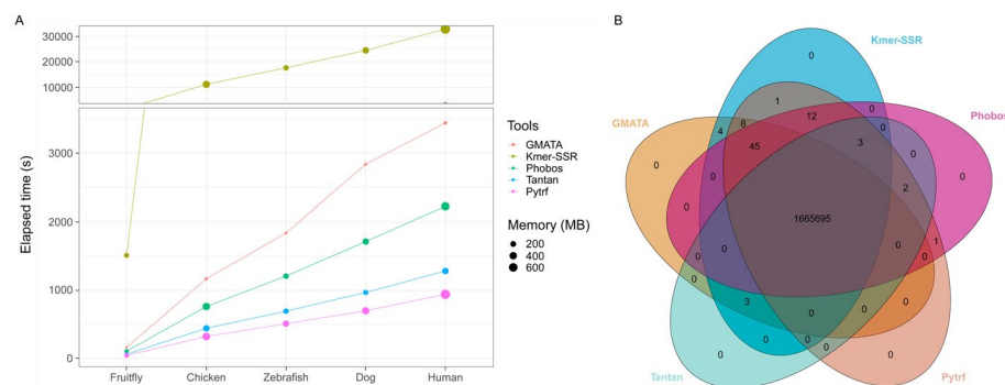
Fig. 4 The performance comparison for finding perfect minisatellites with motif size of 7–100 bp. A comparison of elapsed time and peak memory usage. B venn plot for showing number of intersections between different tools
